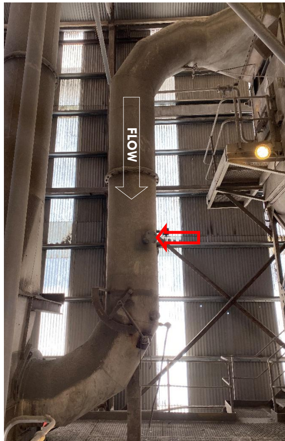
Figure 3: Cement Mill 2 Exhaust Stack sampling plane location
